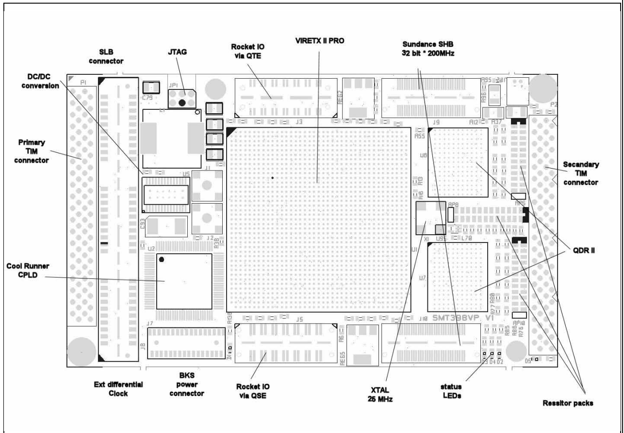
Figure 4: Top View
