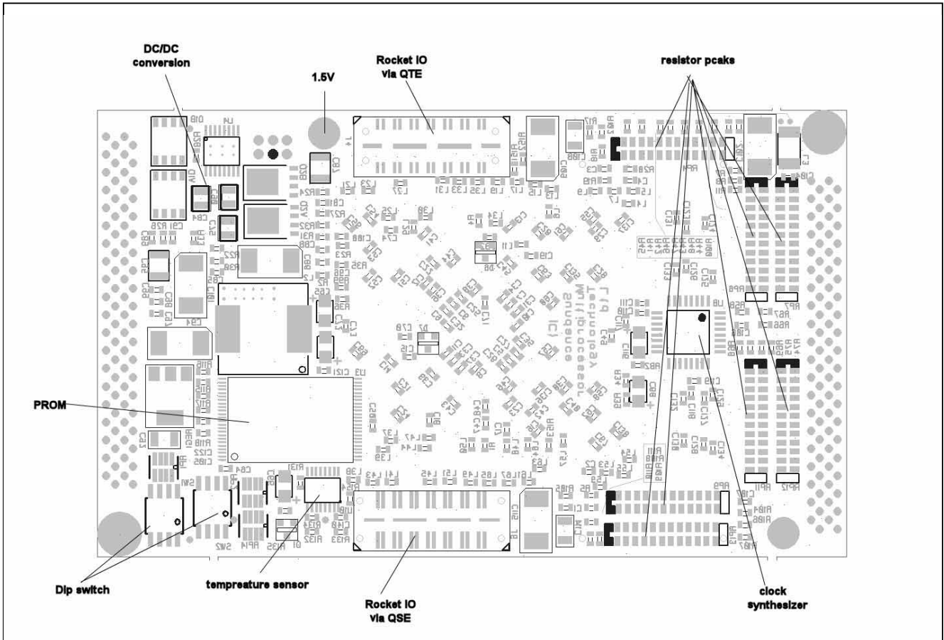
Figure 5: Bottom View
