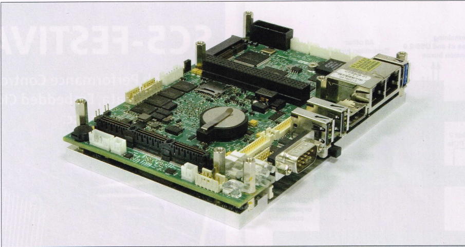
Figure 3. Industry form-factor 3.5" meets PCIe/104 expansion concept
