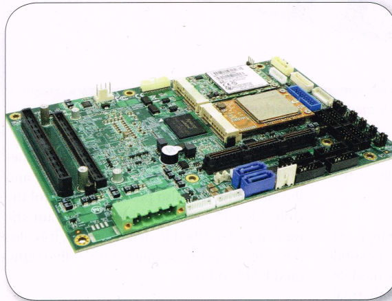
Figure 1. EBX form-factor with PCIe/104 Expansion connector and integrated MiniPCIe for I/O expansion
