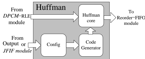
Figure 2.2.7 Huffman module
