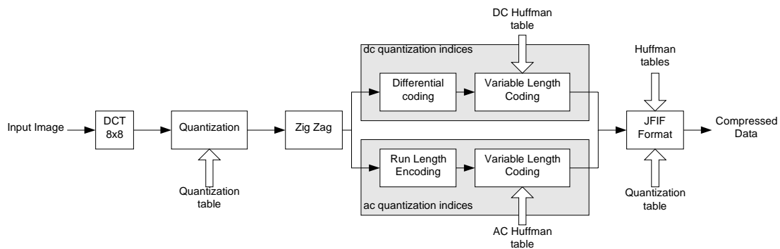
Figure 2.1.0 standard JPEG compression architecture
