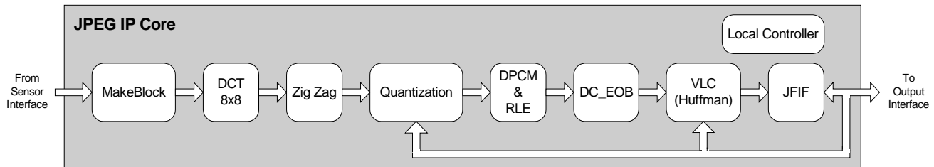
Figure 2.2.0 FC-JPEG04 core design implementation.
