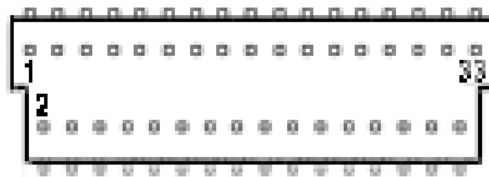
Figure 4 - BKT-133-03-F-V-A – Top View.
