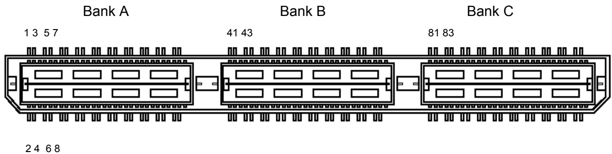
Figure 1 - QTH-060-01-F-D-DP-A (Top View)
