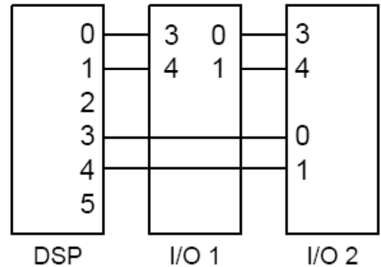
ComPort Connections
