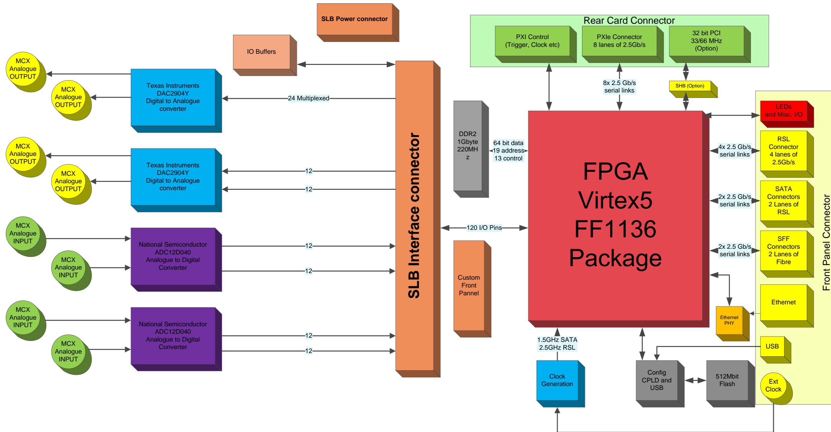
SMT959 Block Diagram
