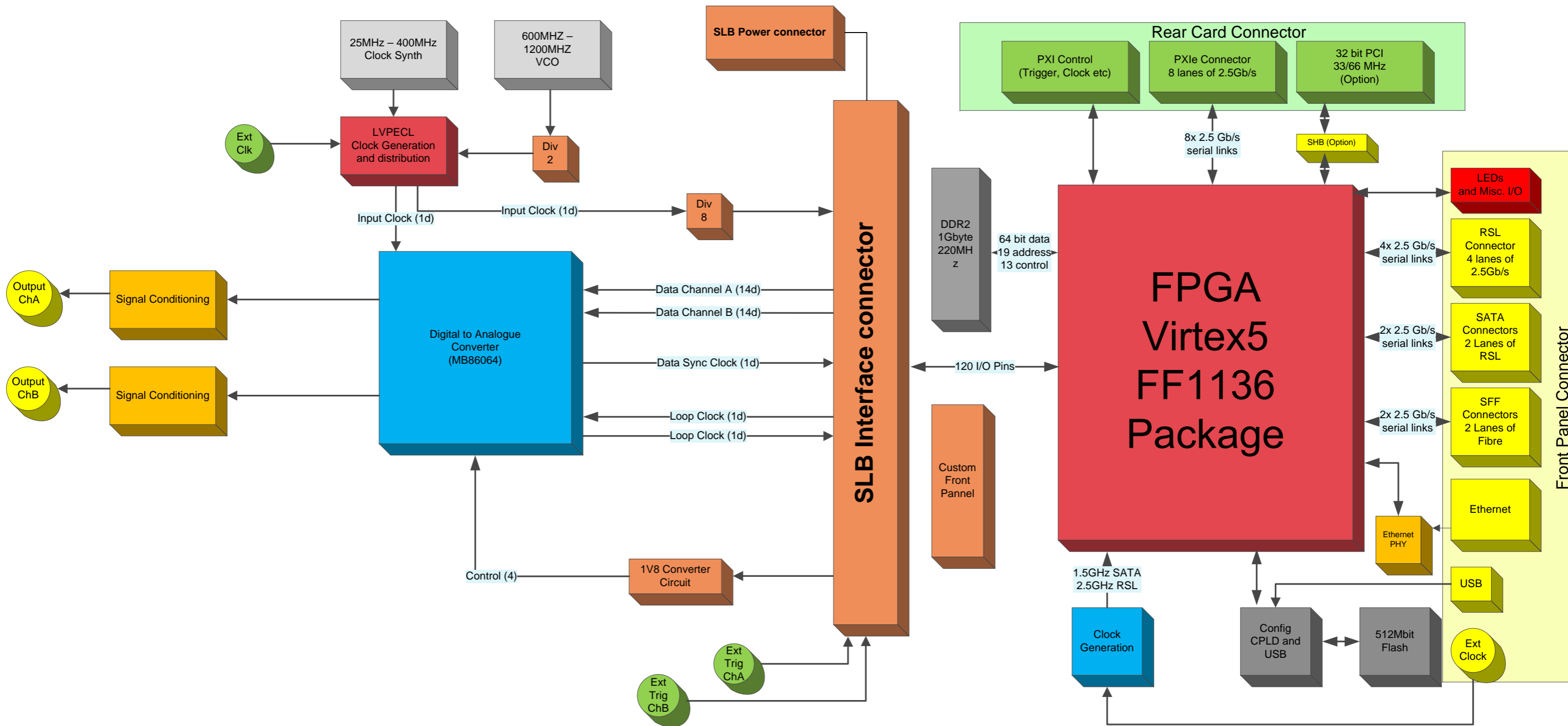
SMT381 Block Diagram
