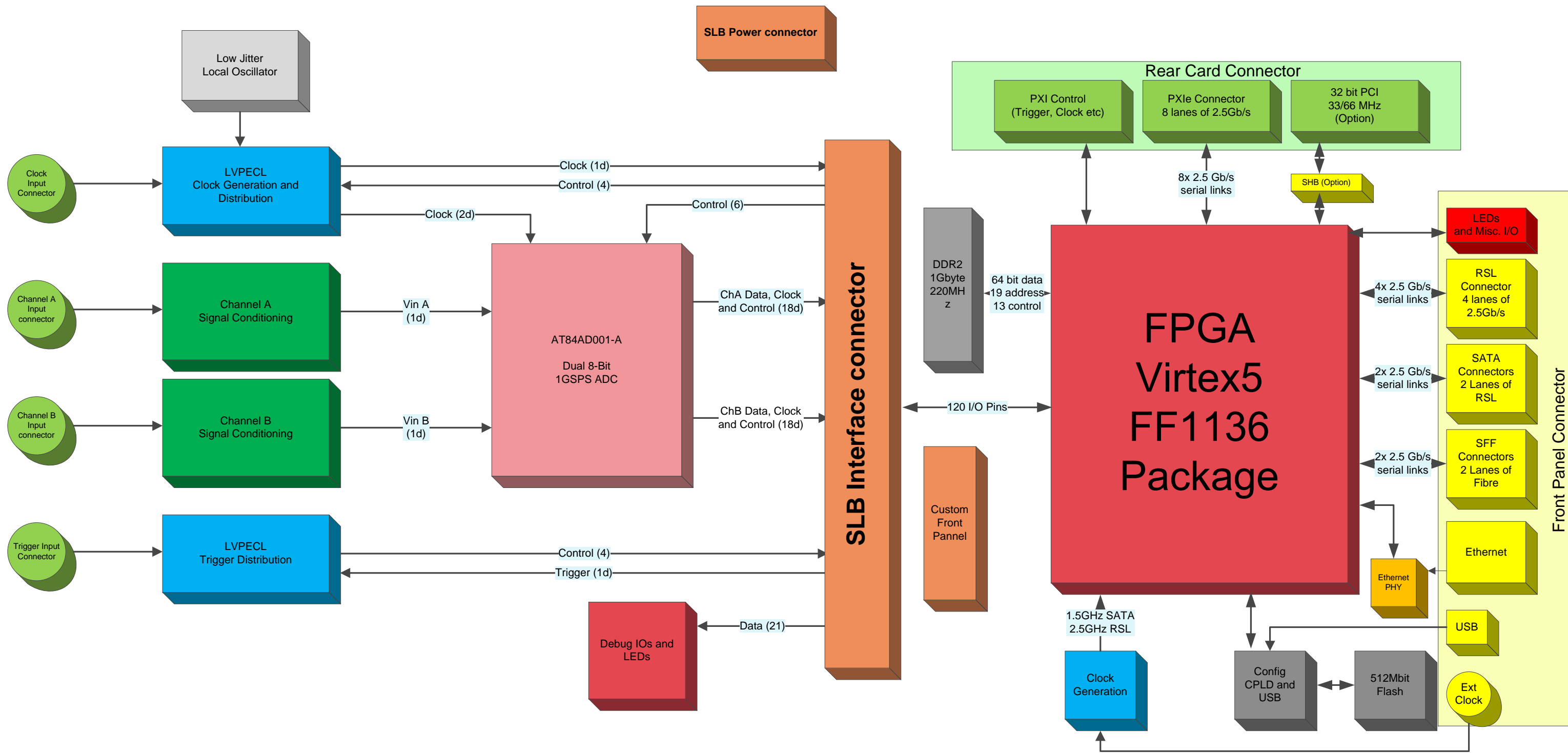
SMT391 Block Diagram
