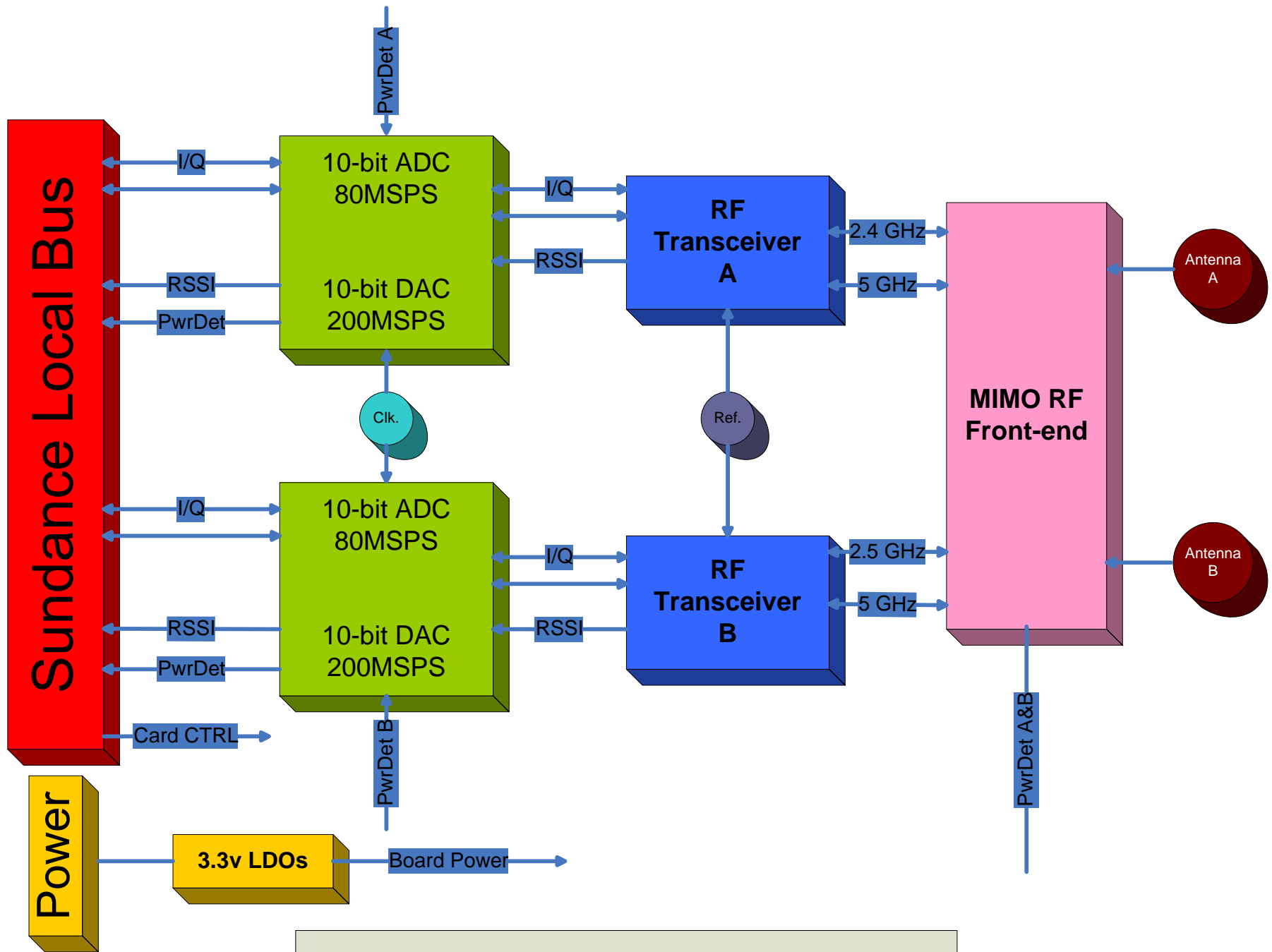
SMT901 Block Diagram
